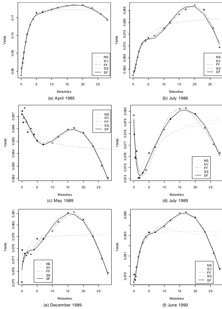
Note: figure 6 shows the McCulloch spot curves observed in six specific months of the sample and exhibits the fitting of the SS, NS, SV, FF and SF models to these curves.
