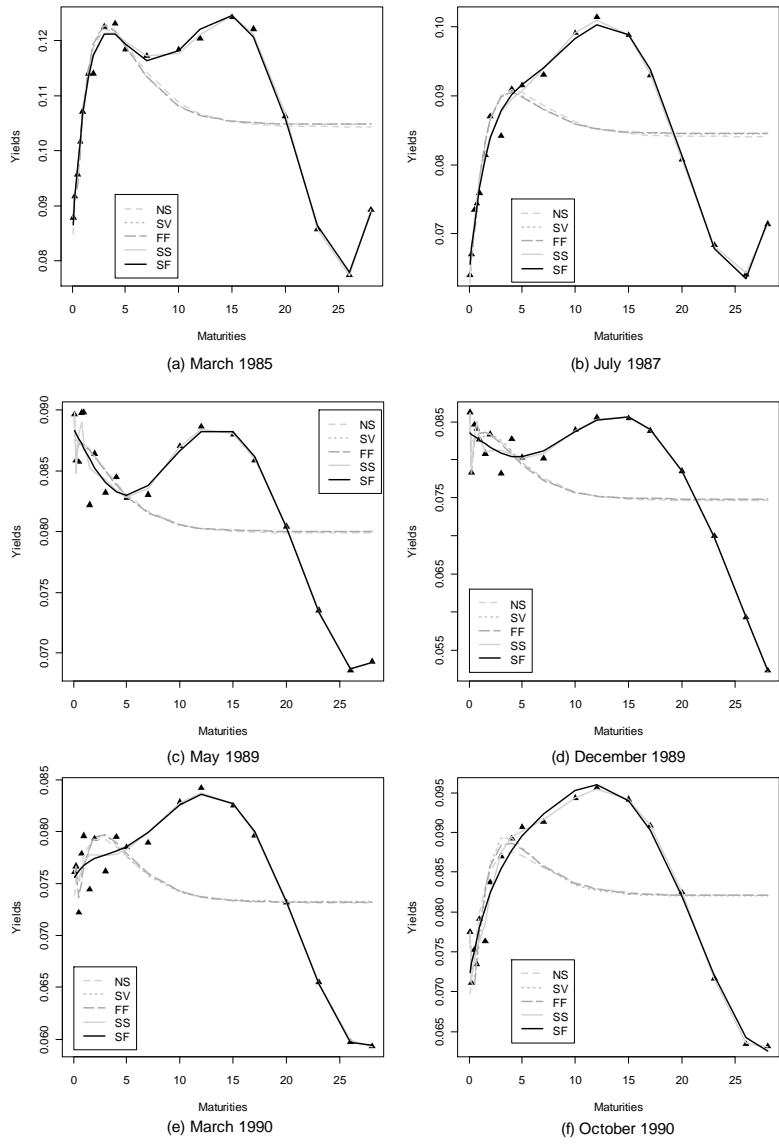
Note: figure 7 shows the McCulloch forward curves observed in six specific months of the sample and exhibits the fitting of the SS, NS, SV, FF and SF models to these curves.
